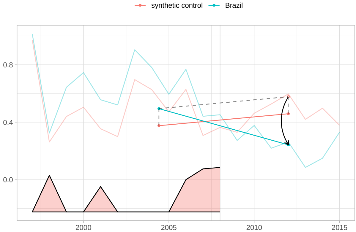
Figure 14: SDiD fit with a Latin American donor pool. Note: Unit = absolute UNGA ideal-point distance to China (points). Standard error = placebo-based (reported in text; not plotted here). Time window = pre-treatment and post-treatment years shown in the plot (treatment in 2009). Treatment definition = Treatment indicator equals 1 from 2009 onward, when China becomes Brazil's top export destination displacing the USA, and 0 before 2009.
